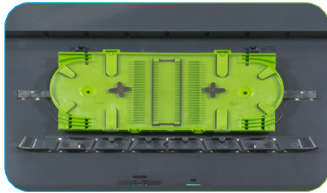
RECEIVES UP TO 2 SPLICE TRAYS 24 FO P/N: 48K724F02298
